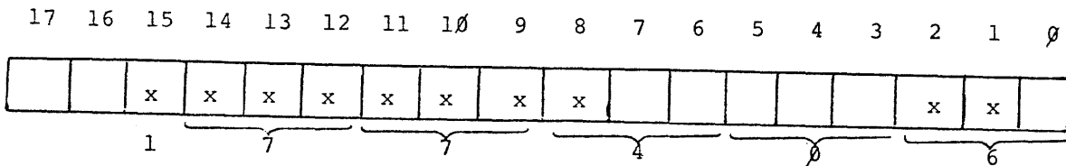
Figure 1-7b Set for RK11 Disk
